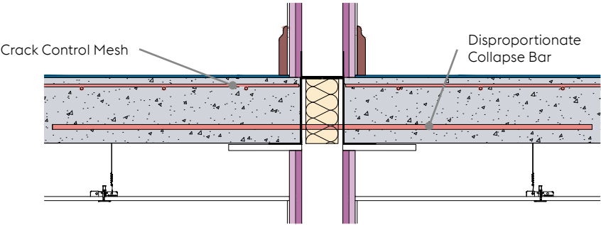
Section at Floor Level with Reinforcement
