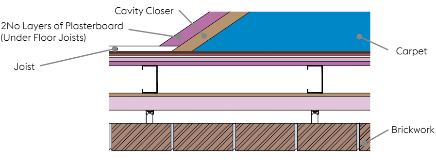
Plan in Floor Build Up
