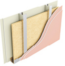
Option 3 2 x 15mm British Gypsum Fireline plasterboard each side, single 100mm stud, 1 x ISOVER 50mm APR 1200 quilt to cavity. O/A width 160mm.
