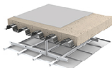
Option 6 Minimum 160mm deep concrete slab (80mm minimum), 5mm Collecta Rubberform, MF ceiling with 1 x 15mm British Gypsum Soundbloc.
