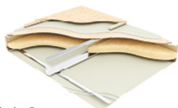
Option 3 Type F9: Three layers of 12.5mm British Gypsum Fireline plasterboard, resilient bars, joists with 1 x ISOVER 50mm APR 1200 quilt to cavity, 15mm plywood, 19mm British Gypsum Plank, 70mm Collecta Deckfon acoustic battens, 18mm V313 chipboard.
