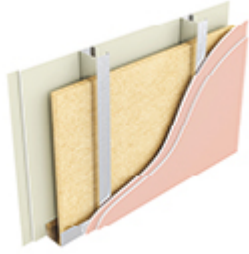
Option 2 2 x 12.5mm British Gypsum Fireline plasterboard each side, single 100mm stud, 1 x ISOVER 50mm APR 1200 quilt to cavity. O/A width 150mm.
