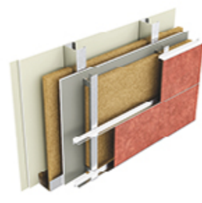
Option 3 Type EC1i: Two layers of minimum 12.5mm British Gypsum Fireline plasterboard, stud with ISOVER 50mm APR 1200 between, sheathing board, Rockwool Duo Slab Insulation, ventilated rainscreen.
