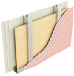
Option 4 3 x 15mm British Gypsum Fireline plasterboard each side, single 100mm stud, 1 x ISOVER 50mm APR 1200 quilt to cavity. O/A width 190mm.
