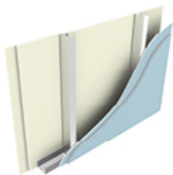
Option 1 2 x 15mm British Gypsum SoundBloc soundboard plasterboard each side, single 100mm stud. O/A width 160mm.
