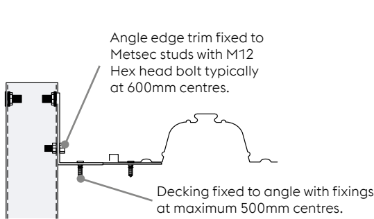
Fixing Edge of Decking to Metsec Wall MF501A
