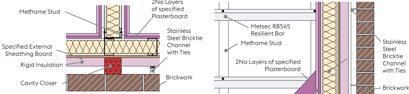
Plan at Junction
