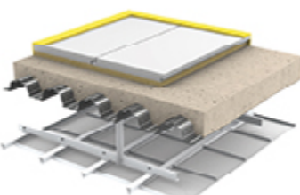
Option 7 (Scotland) Minimum 160mm deep concrete slab (80mm minimum), Collecta Screedboard 30, Metsec MF ceiling with 1 x 15mm British Gypsum Soundbloc.
